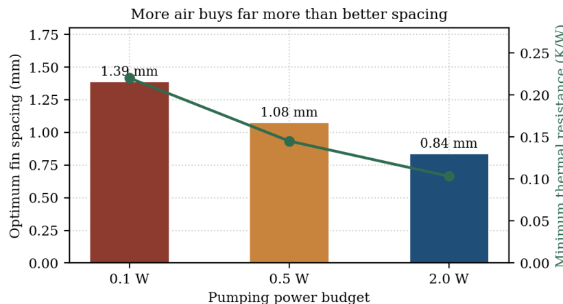
Fig.3: Optimum spacing and minimum achievable resistance against pumping power budget.
