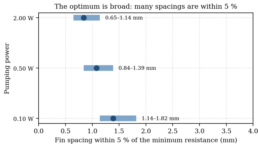
Fig.4: Range of fin spacing within 5 % of the minimum resistance at three power budgets.
