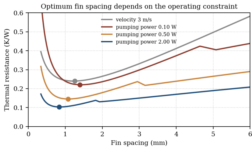
Fig.1: Thermal resistance against fin spacing under four formulations, with each optimum marked.
