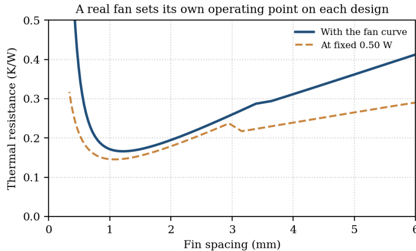
Fig.2: Resistance against spacing with a real fan curve compared with a fixed pumping power.
