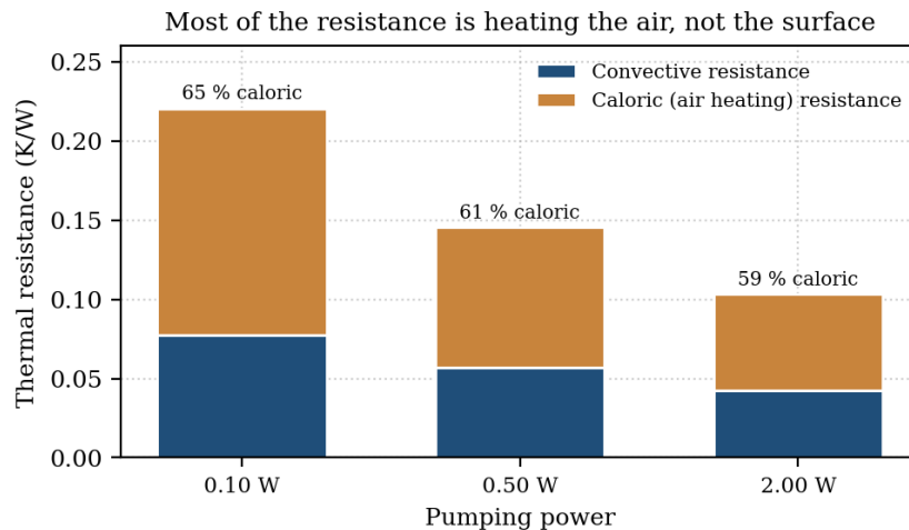
Fig.5: Convective and caloric contributions to minimum thermal resistance.
